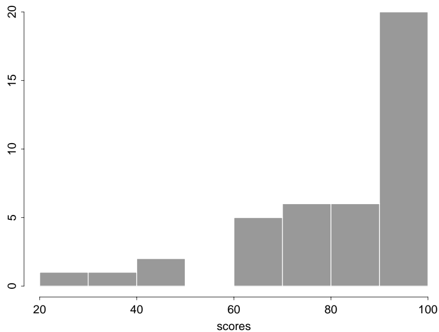
Figure 1: Graphical analysis of Exam grades.
