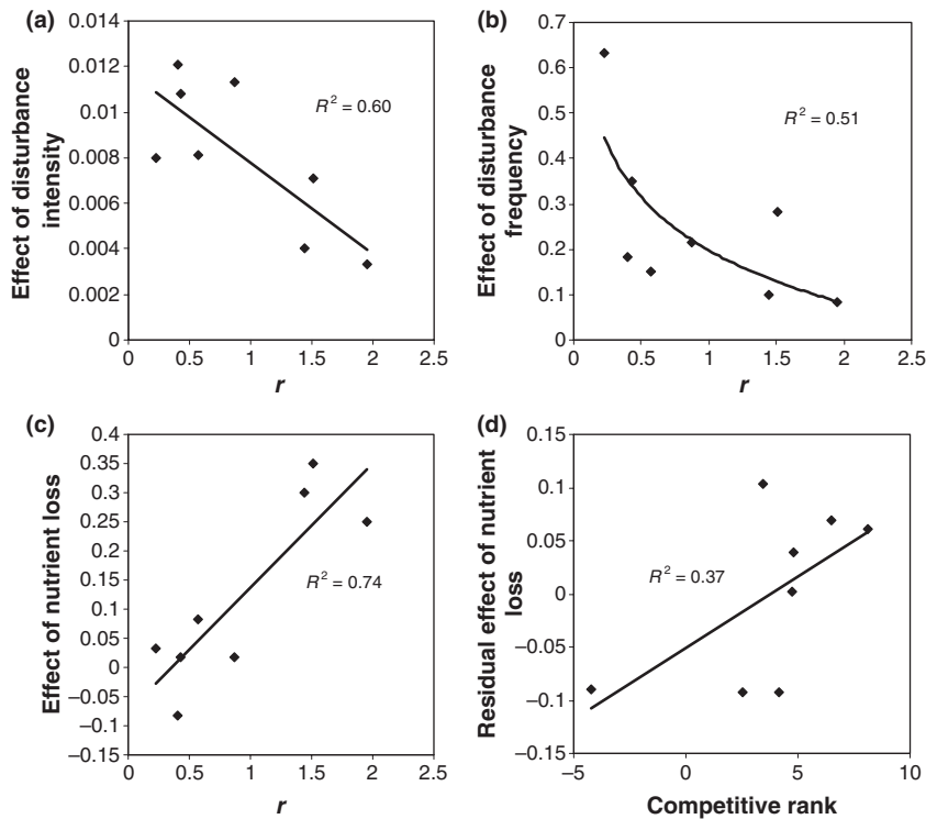
Figure 2 Effects of traits on species' responses to disturbance (a) intensity, (b) frequency and (c,d) effects on productivity. Each panel shows the effects of disturbance in reducing persistence, with high values representing stronger negative effects. Each point represents a single species. Disturbance responses were measured as (a) slope of regression for each species between disturbance intensity and proportion of replicates occupied, (b) the difference between proportion of replicates occupied under low- and high-disturbance frequency and (c,d) the difference between proportion of replicates occupied under high and low nutrients following disturbance. In (d), the response variable is the residual of the relationship between r and the response to productivity (multiple regression R^2 = 0.96 ).
